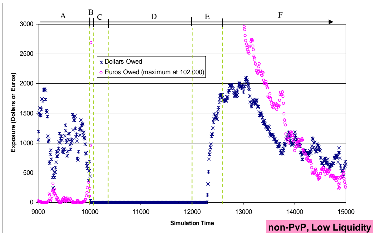
Chart 13: Time series of the FX exposures (Dollars Owed or Euros Owed), in the non-PvP case, with a low level of liquidity in both systems. A large local € bank faces an operational outage between time 10000 and 12000.
