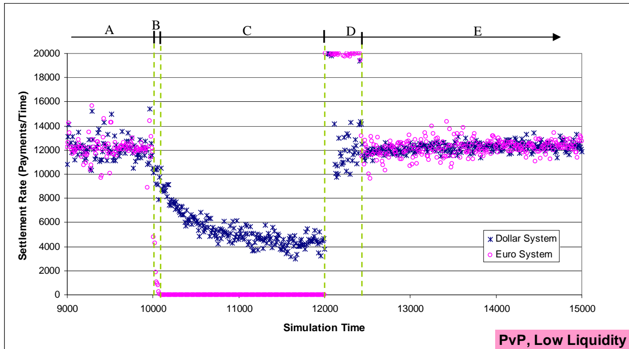
Chart 9: Time series of the settlement rate in the two RTGS systems, in the PvP case, with a low level of liquidity in both systems. A large local €bank faces an operational outage between time 10000 and 12000.
