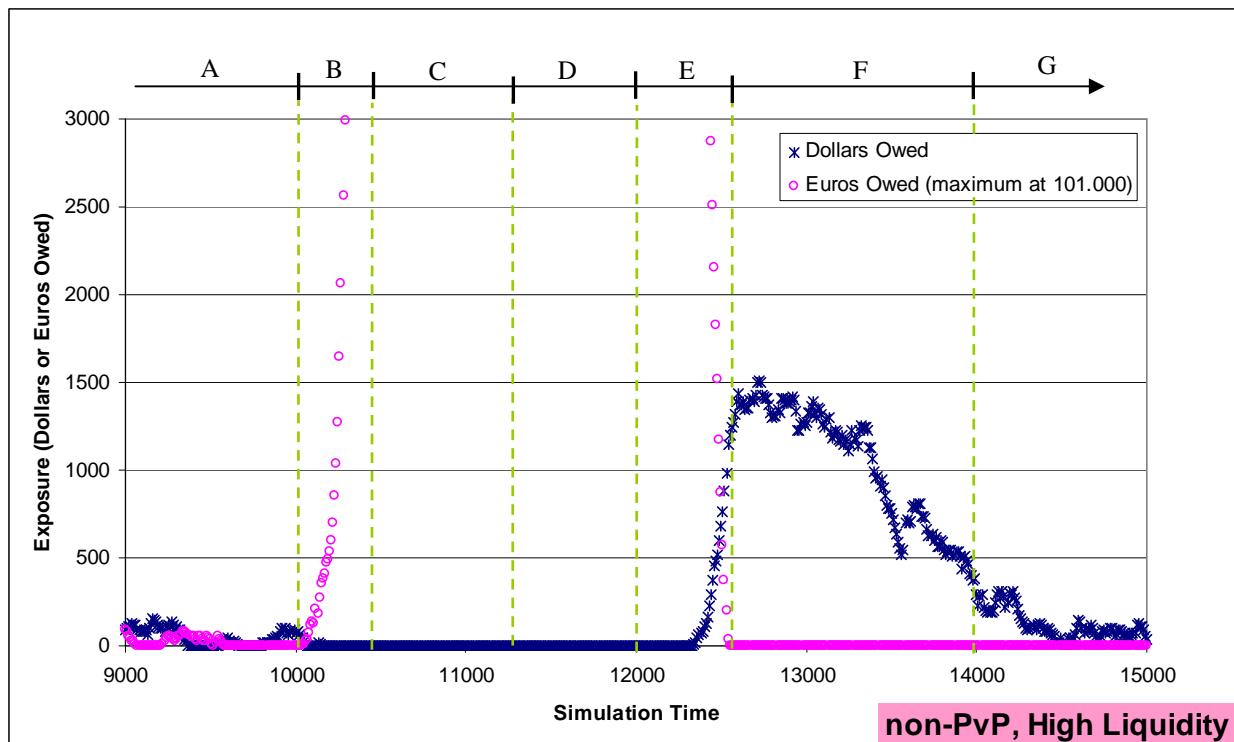
Chart 12: Time series of the FX exposures (Dollars Owed or Euros Owed), in the non-PvP case, with a high level of liquidity in both systems. A large local € bank faces an operational outage between time 10000 and 12000.
