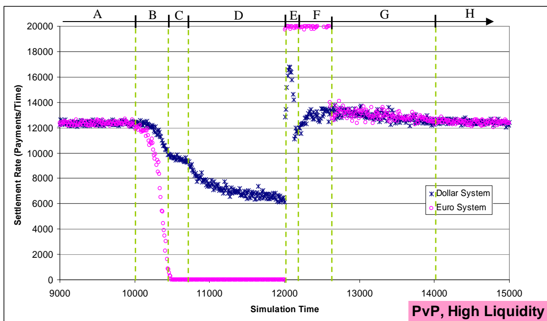
Chart 8: Time series of the settlement rate in the two RTGS systems, in the PvP case, with a high level of liquidity in both systems. A large local € bank faces an operational outage between time 10000 and 12000.
