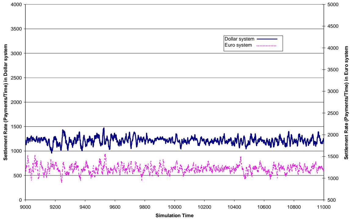
Chart 6: Time series of the settlement rate in the two systems. non-PvP case
