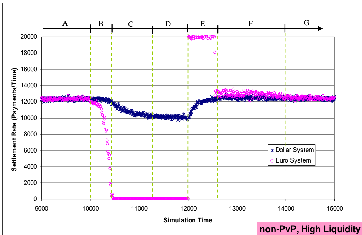
Chart 10: Time series of the settlement rate in the two RTGS systems, in the non-PvP case, with a high level of liquidity in both systems. A large local € bank faces an operational outage between time 10000 and 12000.
