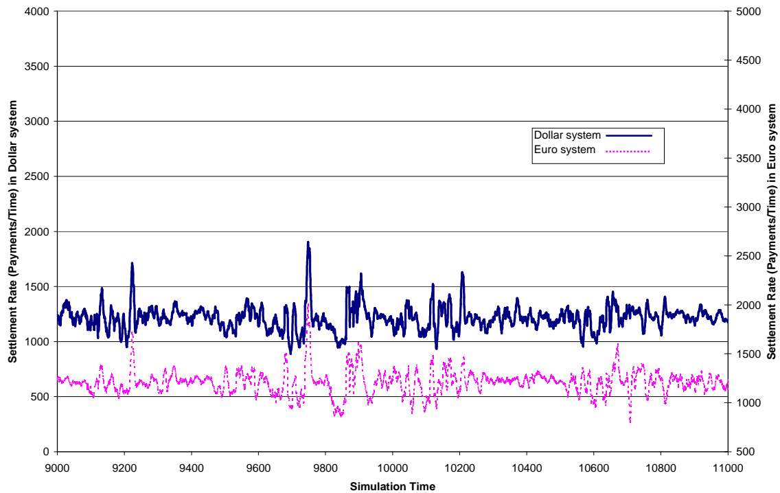
Chart 7: Time series of the settlement rate in the two systems. PvP case
