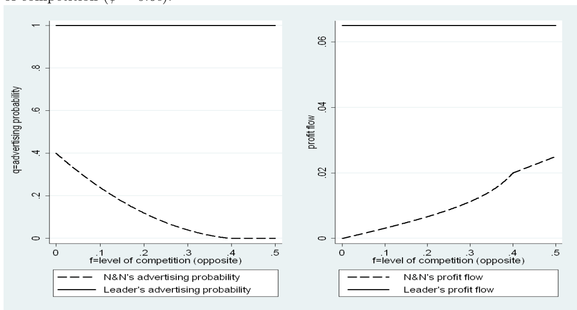
Figure 3: Leader's and Neck and neck's advertising probabilities and profits as a function of competition ( \phi = 0.6\epsilon ):
