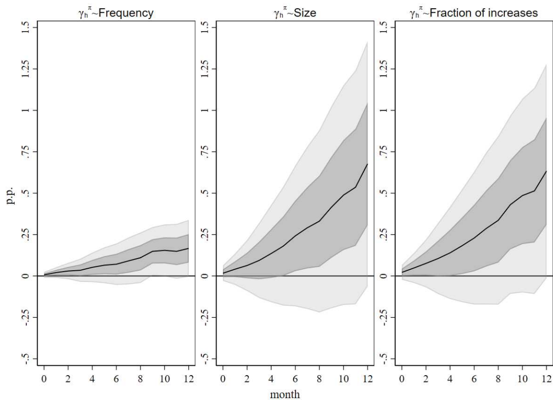
Figure 6: Counterfactual inflation rate responses to a negative oil supply shock: high inflation period relative to low inflation period
