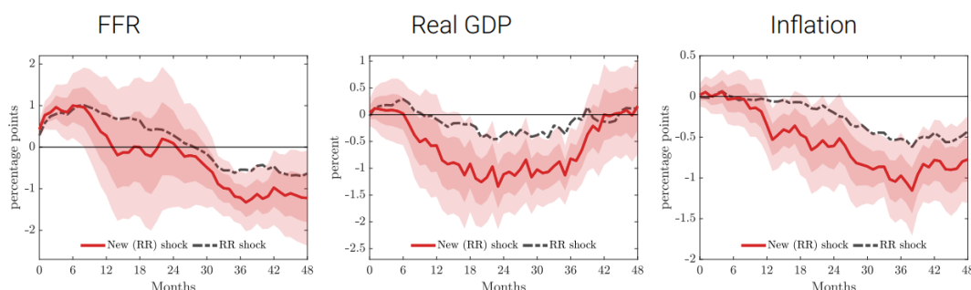
Figure 1: Comparing the effects of new and RR monetary policy shocks on the economy
