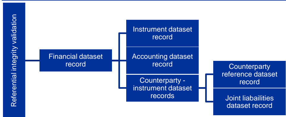
Figure 2 Referential integrity validation path for transmission of a financial dataset record
