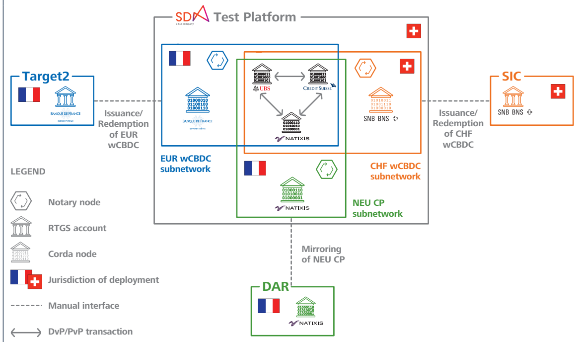
FIGURE 2 – Experimental architecture
