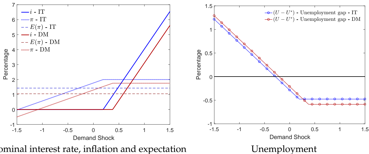
Figure 2: Equilibrium for the Inflation Targeting vs. Dual Mandate
