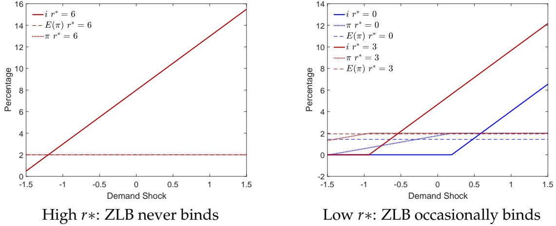
Figure 1: Equilibrium for inflation targeter for different values of r^*
