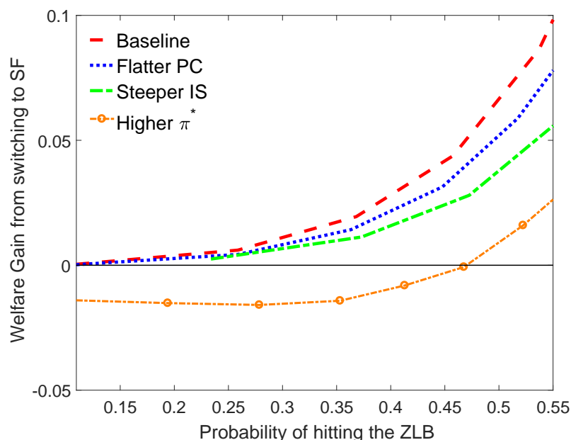
Figure 8: Welfare Gain - Demand shocks
