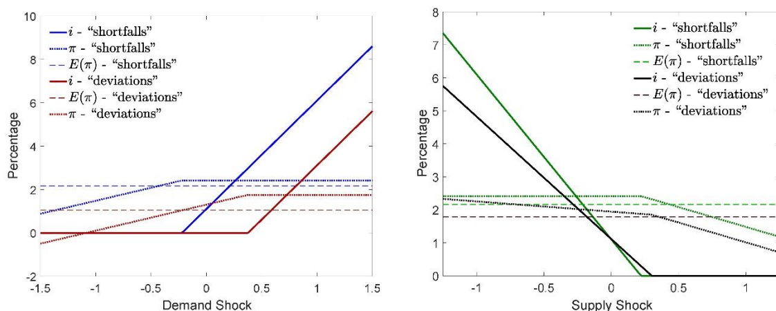
The Figure depicts different equilibrium interest rate, inflation and inflation expectations in the presence of demand (LHS) and supply (RHS) shocks for a Central Bank minimizing "deviations" or "shortfalls" of inflation and unemployment from their target.
